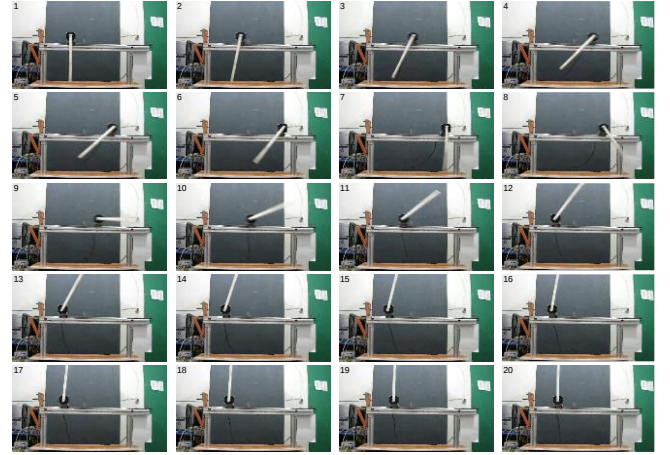
Fig. 14- Snapshots of the optimal swing up manoeuvre
