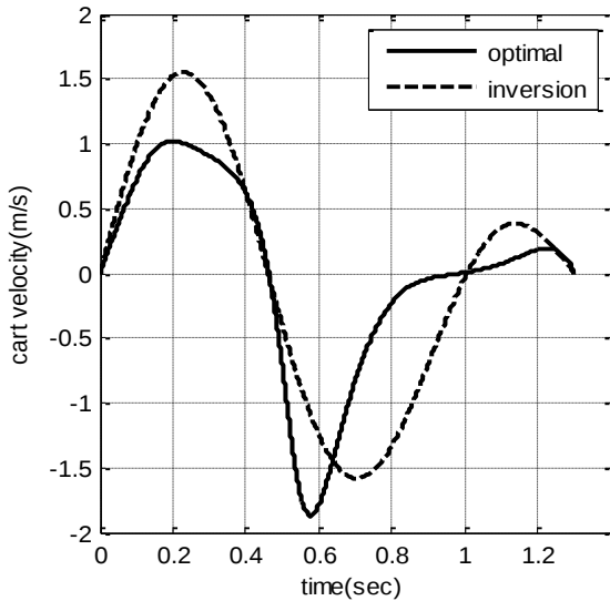
Fig. 5- Linear velocity of cart
