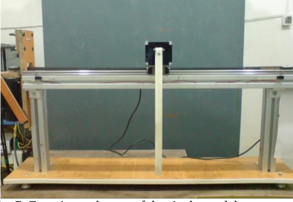
Fig. 7- Experimental setup of the single pendulum on a cart
