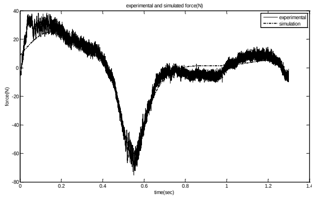
Fig. 18- Experimental and simulated force for optimal swing up
