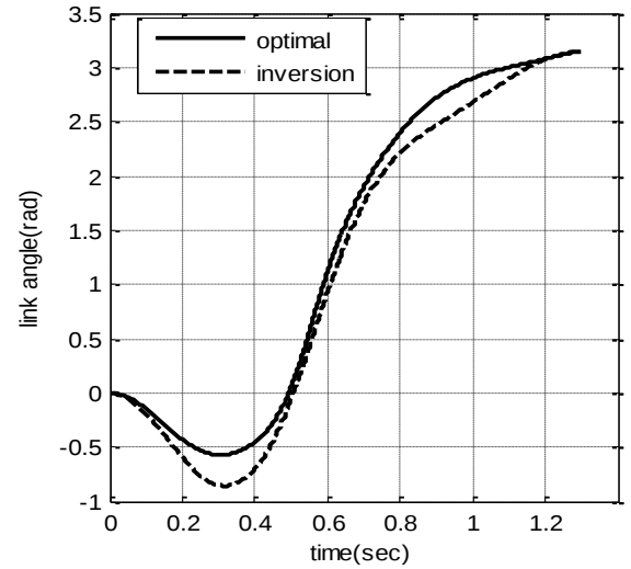
Fig. 2- Angular position of link
