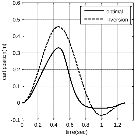
Fig. 4- Linear position of cart
