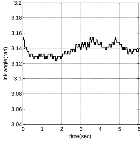
Fig. 12 - Link angle in upright position
