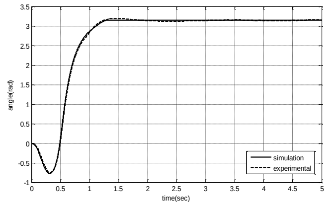
Fig. 15- Link angle for optimal swing up
