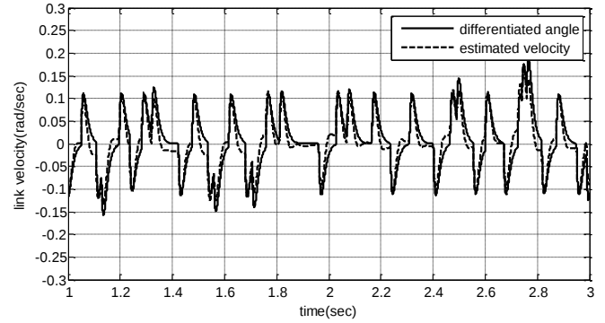
Fig. 9- Differentiated angular position and estimated angular velocity
