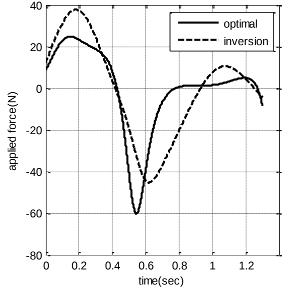
Fig. 6- Applied force to the cart
