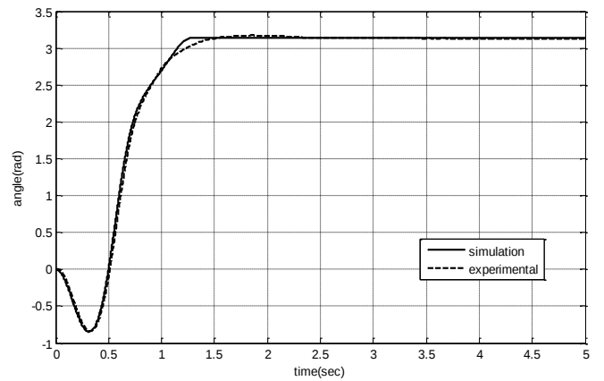
Fig. 16- Link angle for inversion-based swing up
