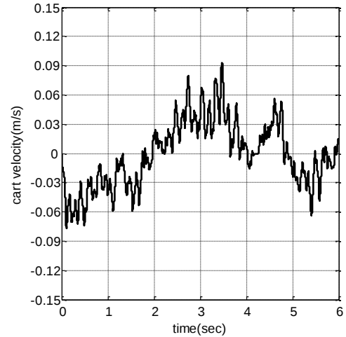
Fig. 11- Cart velocity in upright position
