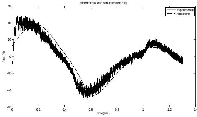
Fig. 17- Experimental and simulated force for inversion-based swing up
