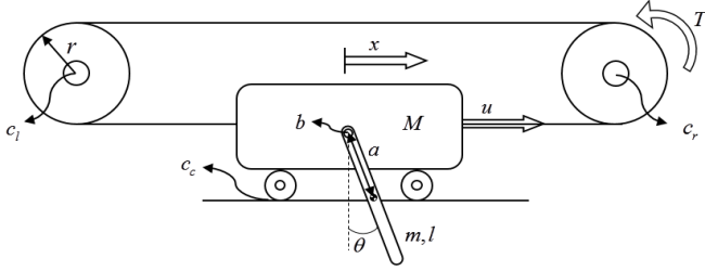
Fig. 1- Schematic model of SIP
