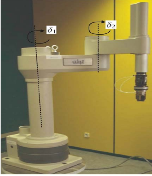
Fig 5 SCARA robot
