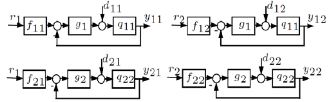
Fig 2 Two-degrees-of-freedom control system MIMO structure
