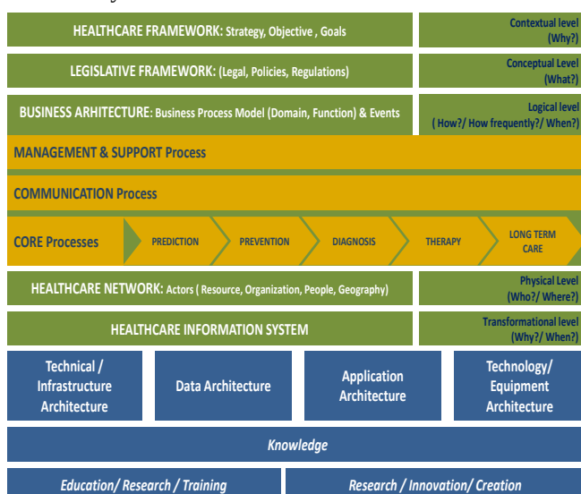
Figure 3. Enterprise Architecture for e-Health system (Costetchi, N. et al, 2013)
