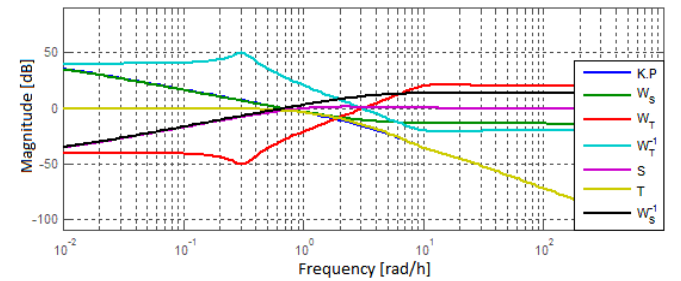
Fig. 8. Bode characteristics for the dilution rate – organic substrate concentration control channel.
