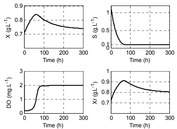
Fig. 3. The simulation results of the open loop model.
