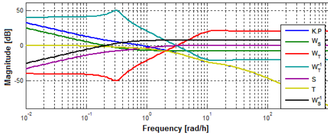
Fig. 10. Bode characteristics for the aeration rate – dissolved oxygen concentration control channel.
