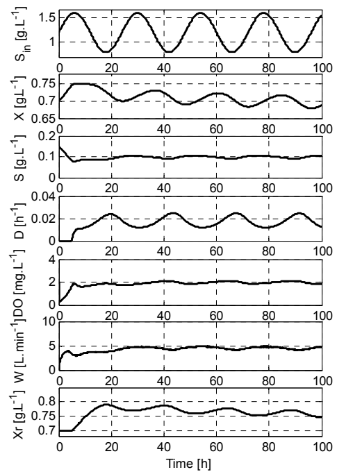
Fig. 22. The simulation results in the presence of the sinusoidal variation of the disturbance S_{in} .
