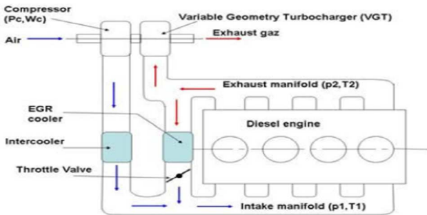
Fig. 1. Turbocharged Diesel Engine.
