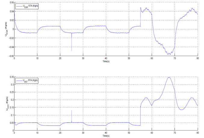
Fig. 5. Control inputs U_{EGR} and U_{VGT} for the STA with Additive leakage time varying faults and multiplicative loss-of-effectiveness time varying faults in EGR and VGT actuators.
