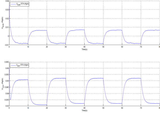
Fig. 3. Control inputs U_{EGR} and U_{VGT} for the STA with only 20 % parametric uncertainties in the TDE air path model.
