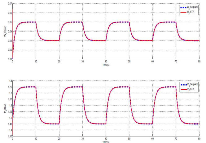
Fig. 2. W_c and P_2 tracking performance for the STA with only 20 % parametric uncertainties in the TDE air path model.
