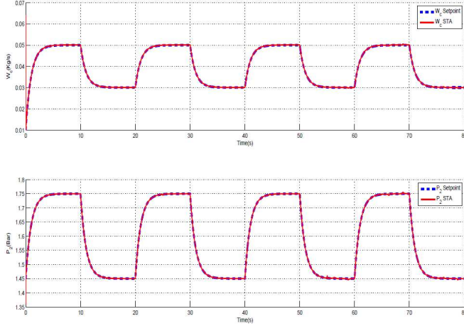
Fig. 6. W_c and P_2 tracking performance for the STA with Additive leakage time varying faults and multiplicative loss-of-effectiveness time varying faults in EGR and VGT actuators [improved gains].
