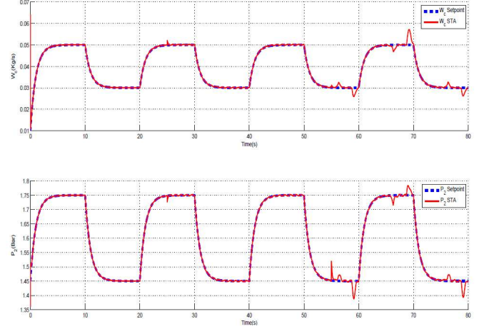
Fig. 4. W_c and P_2 tracking performance for the STA with Additive leakage time varying faults and multiplicative loss-of-effectiveness time varying faults in EGR and VGT actuators.
