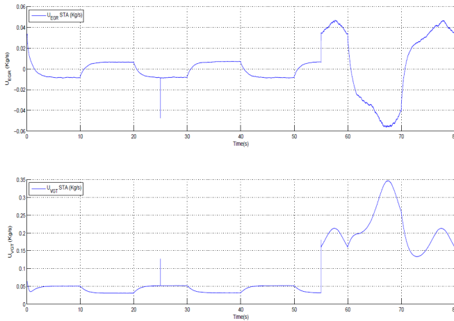
Fig. 7. Control inputs U_{EGR} and U_{VGT} for the STA with Additive leakage time varying faults and multiplicative loss-of-effectiveness time varying faults in EGR and VGT actuators [improved gains].
